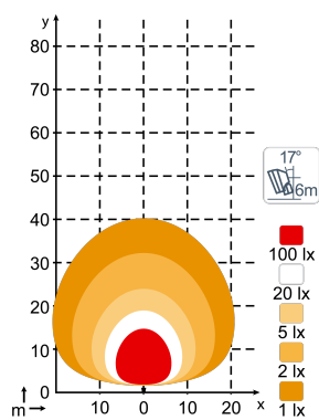
N4701 20160lm Diffused
