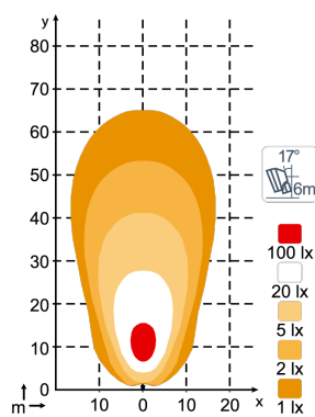
N4701 25200lm Flood
