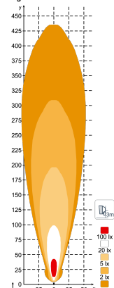
N4701 25200lm High Beam
