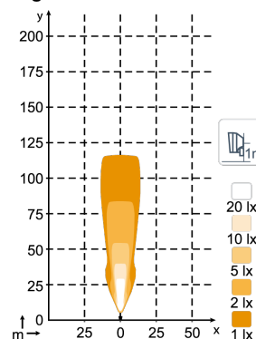
N4405 QD, N4406 2100lm High Beam
