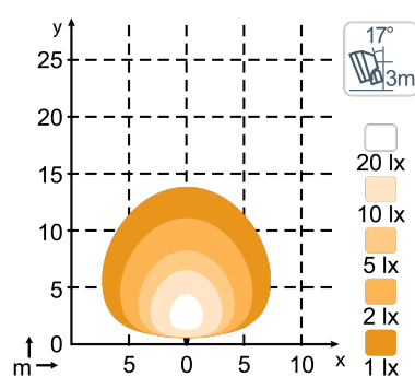
N4405 QD, N4406 1680lm Diffused
