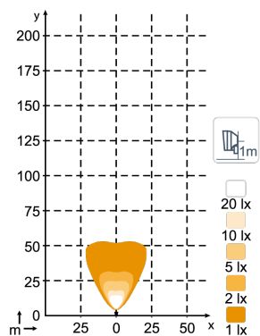
N4405 QD, N4406 2100lm Low Beam
