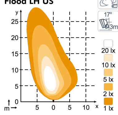
N7301 2600lm Flood LH US
