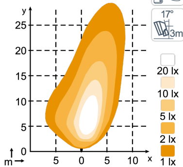
N7301 2600lm Flood RH US
